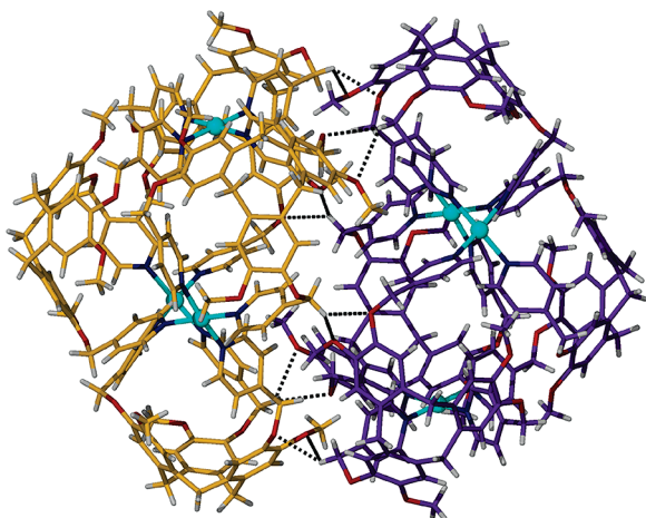
Figure 6. Detail from the crystal structure of [\text{Pd}_3(\mathbf{3})_4](\text{NO}_3)_6 \cdot n(\text{DMSO}) \cdot m(\text{H}_2\text{O}) , showing two of the [\text{Pd}_3(\mathbf{3})_4]^{6+} superbowl hydrogens-bonding together in the solid state.
