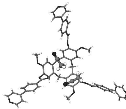
Figure 3. Detail from the crystal structure of 5 \cdot 3^{1/3}\text{MeCN} \cdot \frac{1}{3}\text{H}_2\text{O} showing host–guest interactions between 5 and \text{CH}_3\text{CN} .
