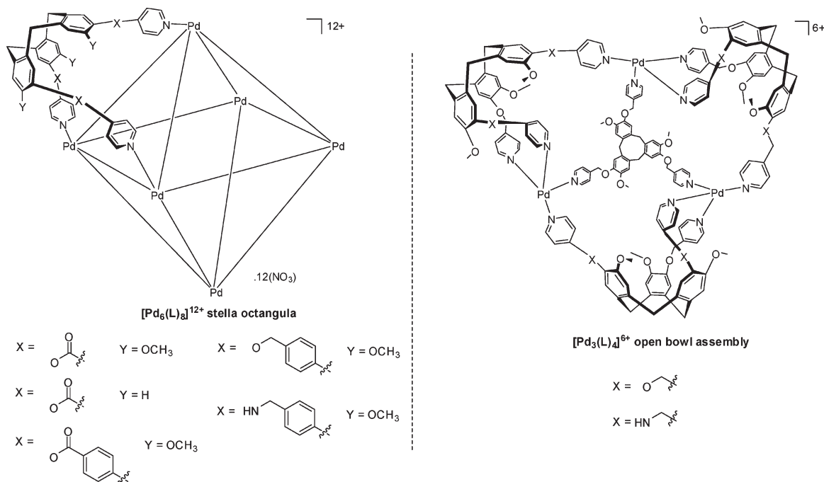
Scheme 3. Schematic Giving a Summary of the Formation of Stella Octangula or Open-Bowl Assemblies with the Different Ligands 1–7
