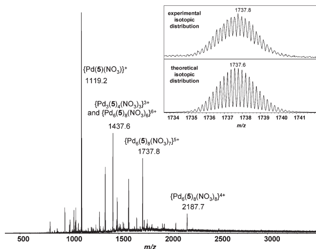
Figure 4. Electrospray mass spectrum of 5 and \text{Pd}(\text{NO}_3)_2 in DMSO. Inset: Theoretical and experimental isotopic distribution patterns for the \{\text{Pd}_6(\mathbf{5})_8(\text{NO}_3)_{12}\}^{5+} peak.
